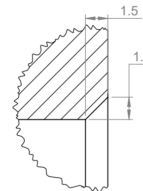
DETAIL H SCALE 4 : 1
