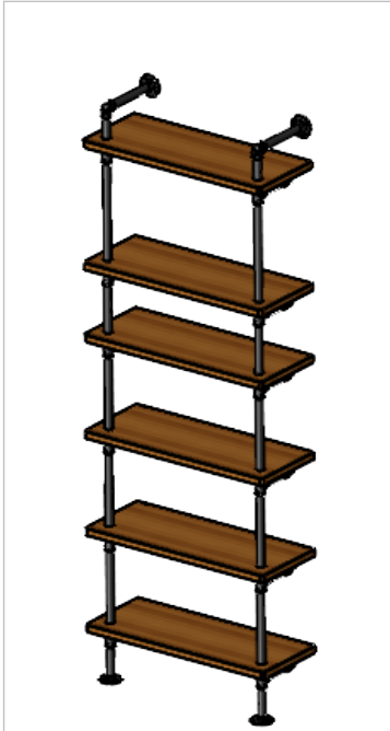
GA-SHELF LEFT-01 SCALE 1:30
