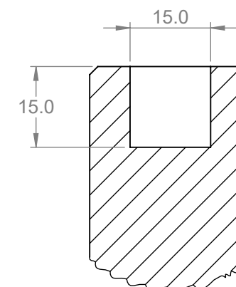
DETAIL F SCALE 1 : 1
