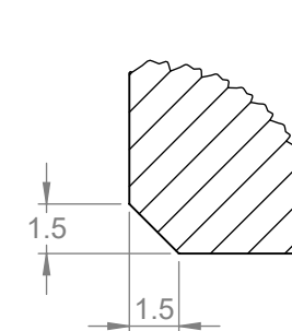
DETAIL I SCALE 4 : 1
