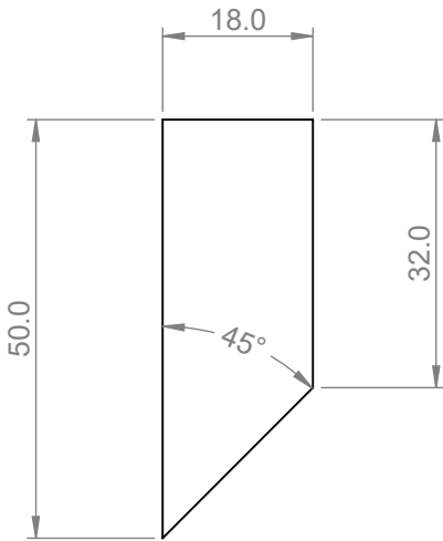
DETAIL G SCALE 1 : 1
