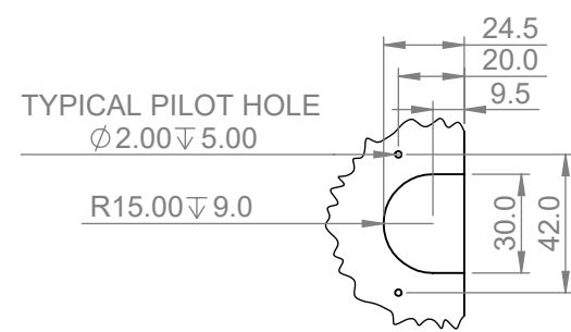
DETAIL I SCALE 2 : 5
