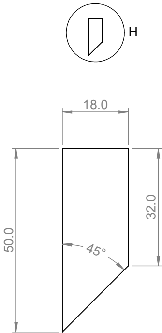
DETAIL H SCALE 1 : 1
